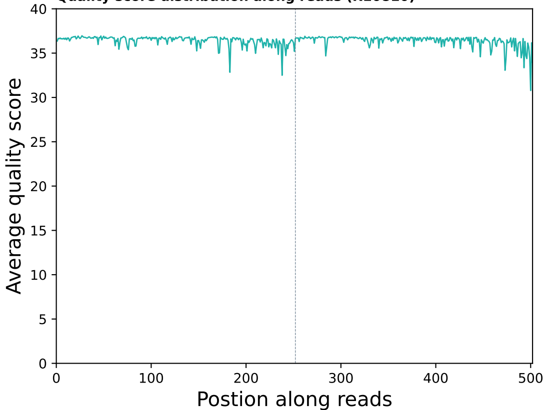
Quality score distribution along reads (R10810)
